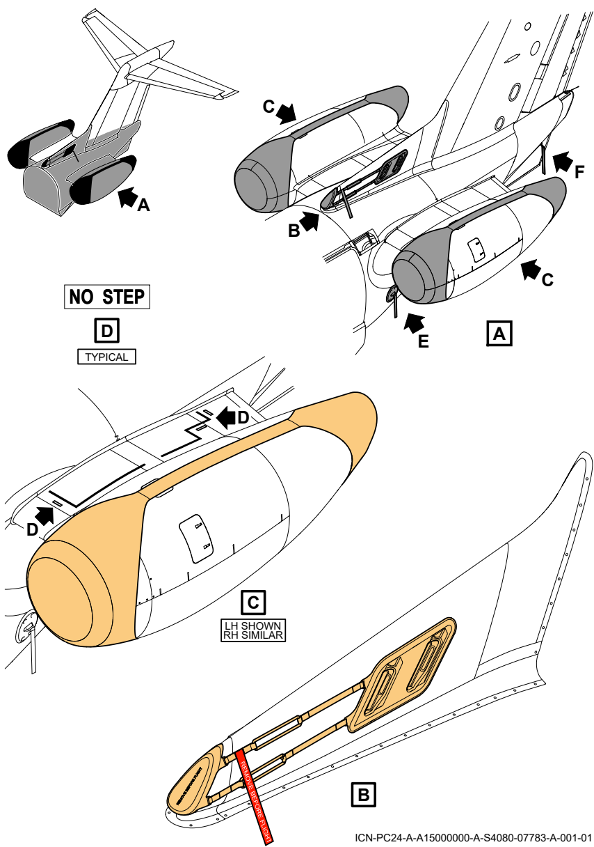
Figure 2-8-1: Parking - Upper Rear Fuselage Covers
