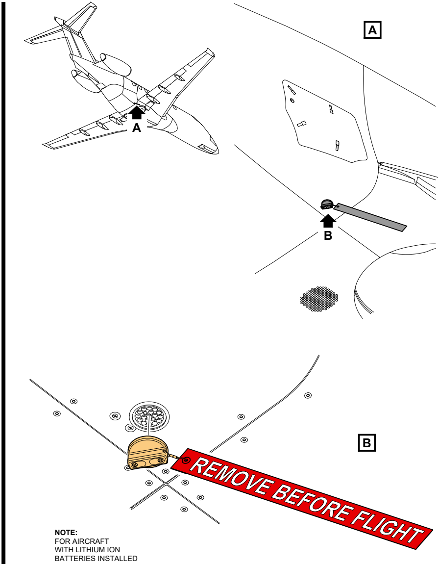
Figure 2-8-5: Parking - Lithium Ion Battery 2 - Vent cover
