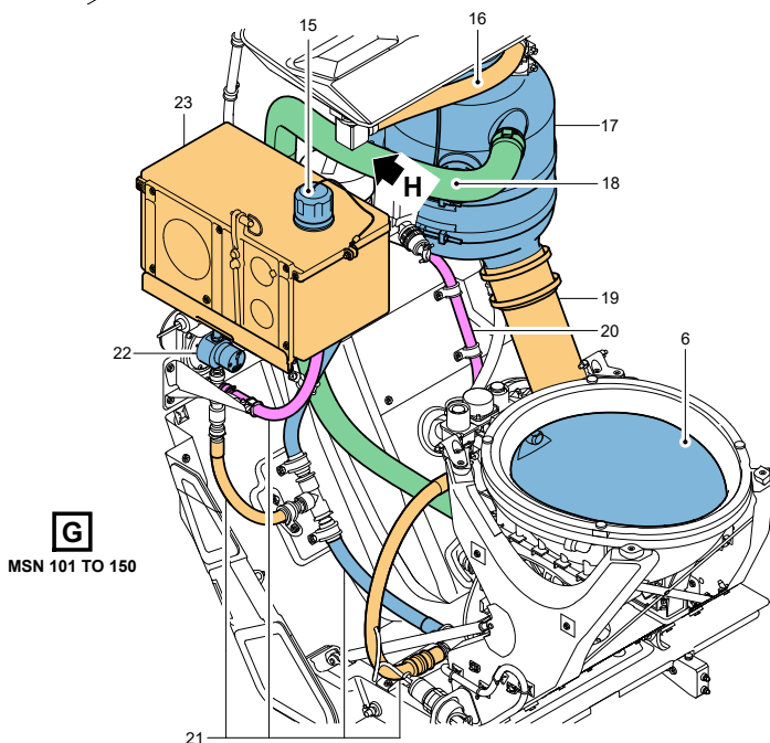
Figure 2-12-1: Water and waste system - Clean (Sheet 3 of 4)
