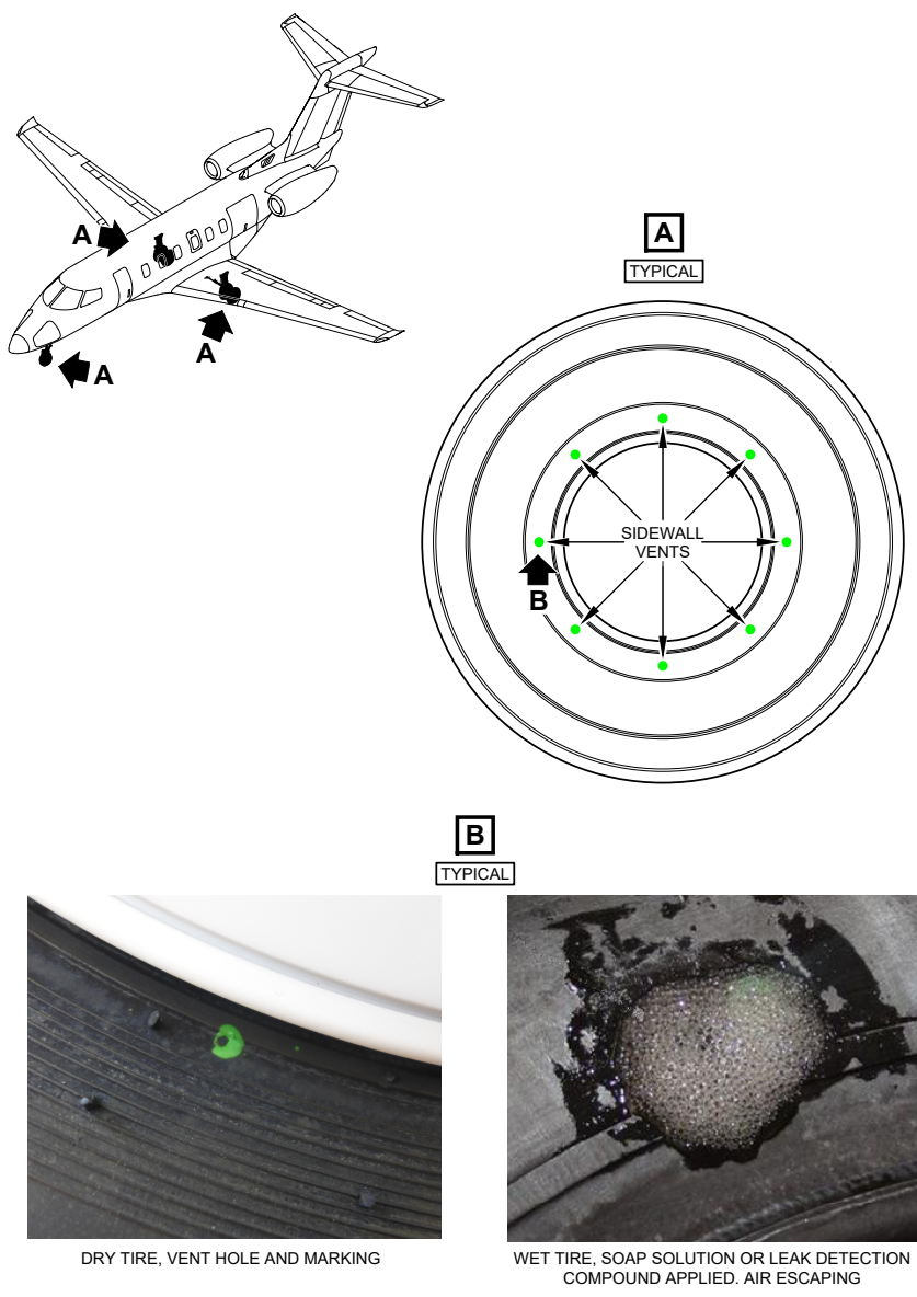
Figure 2-2-2: Tires - Markings
