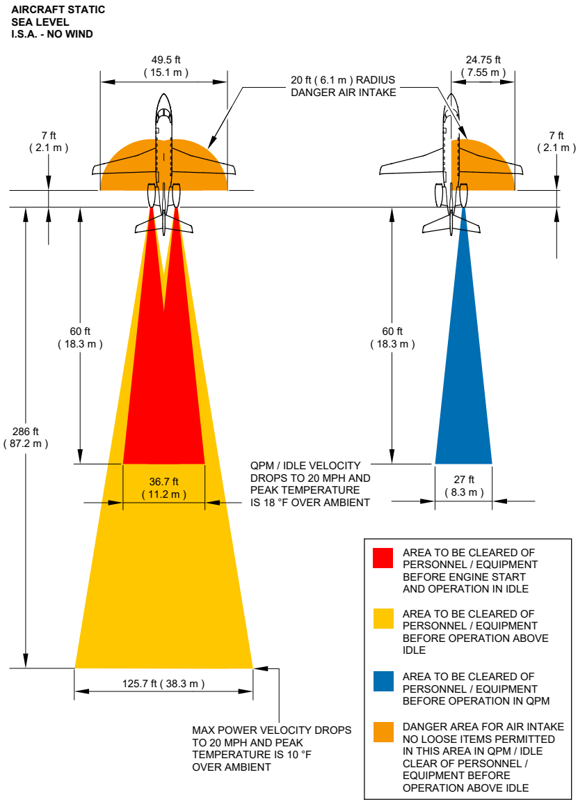
Figure 0-1-3: Danger Areas
