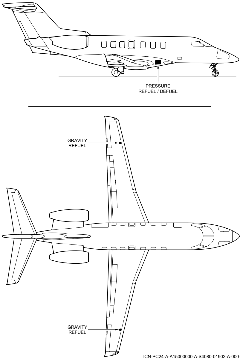
Figure 2-5-1: Fuel System - Refueling Points
