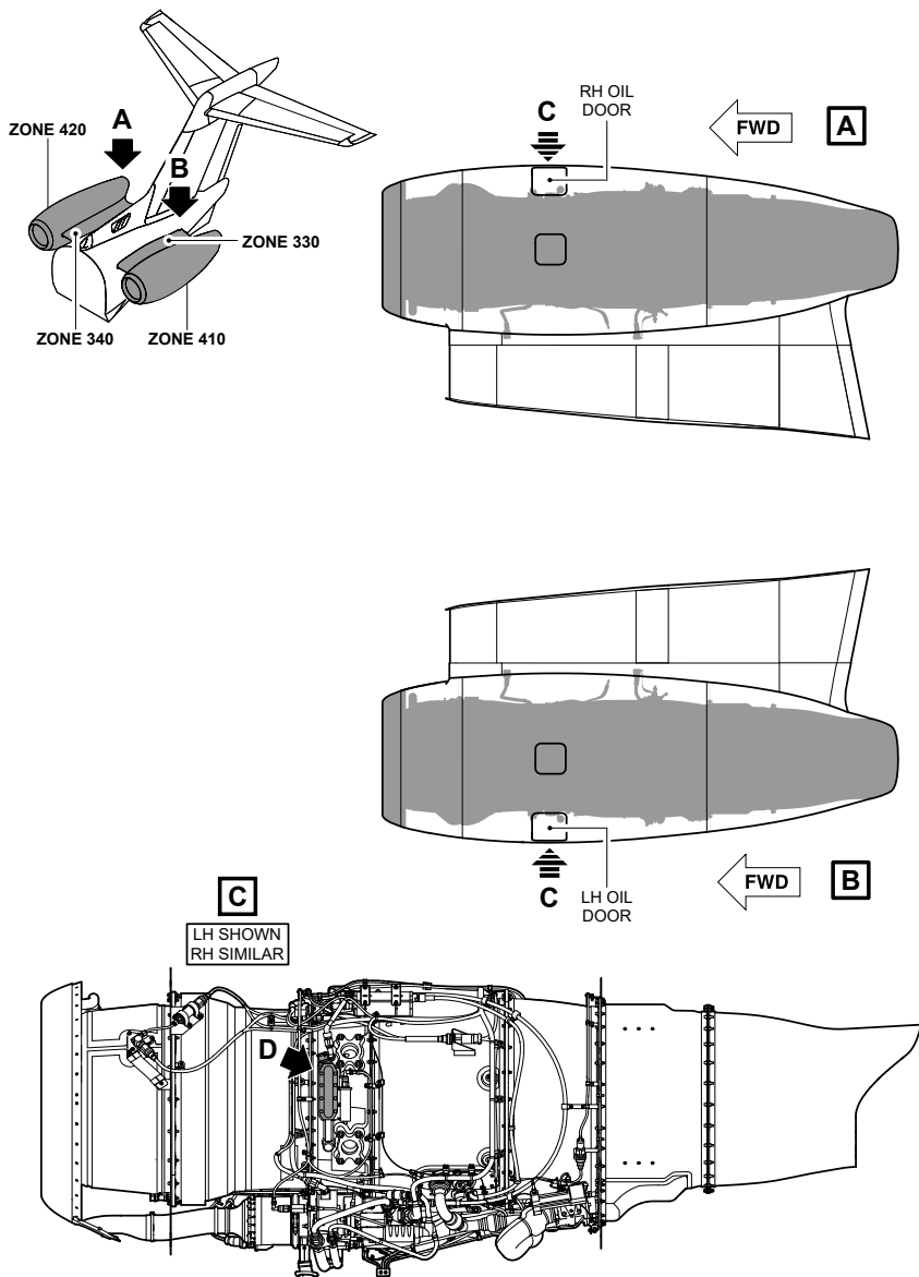
Figure 2-6-1: Engine oil - Fill (Sheet 1 of 2)
