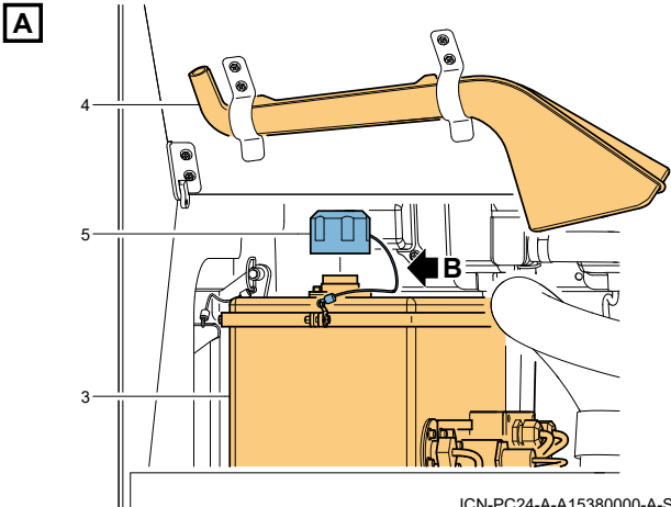
Figure 2-11-2: Water tank - Fill using the funnel (Sheet 1 of 2)
