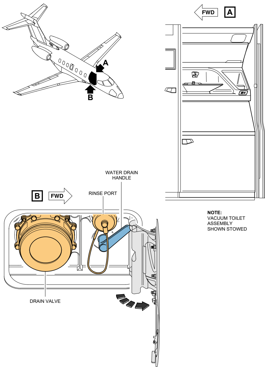
Figure 2-11-1: Vacuum Waste System - Component Location
