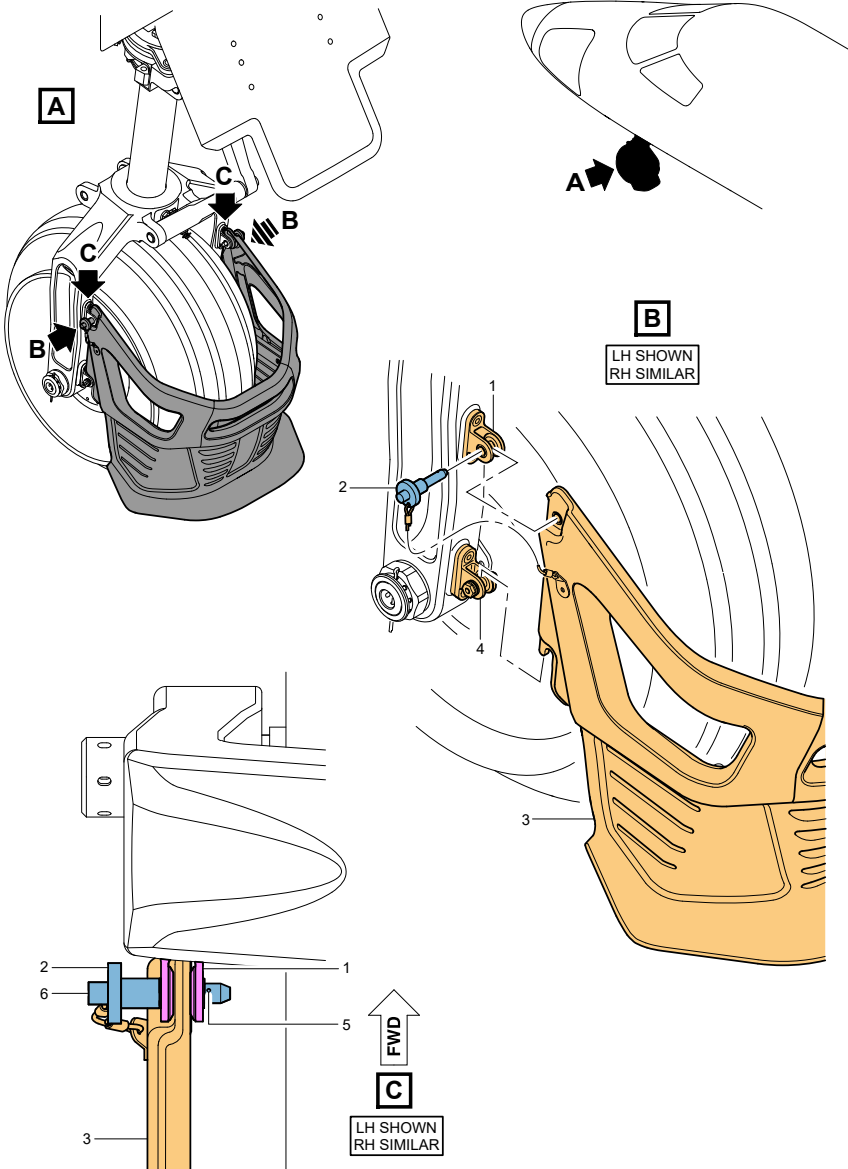
Figure 2-3-1: Quick-release stone guard - Remove and install
