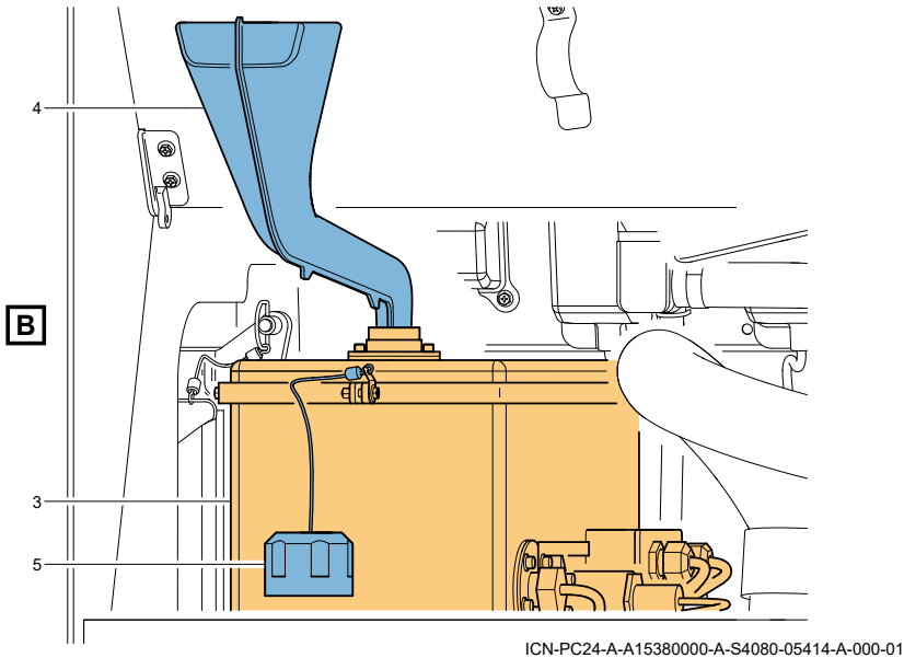
Figure 2-11-2: Water tank - Fill using the funnel (Sheet 2 of 2)
