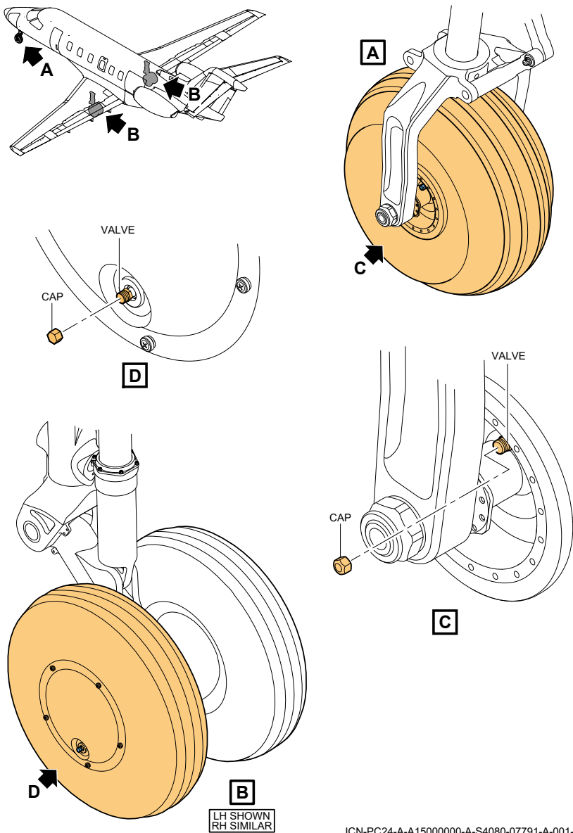
Figure 2-2-1: Tires - Fill
