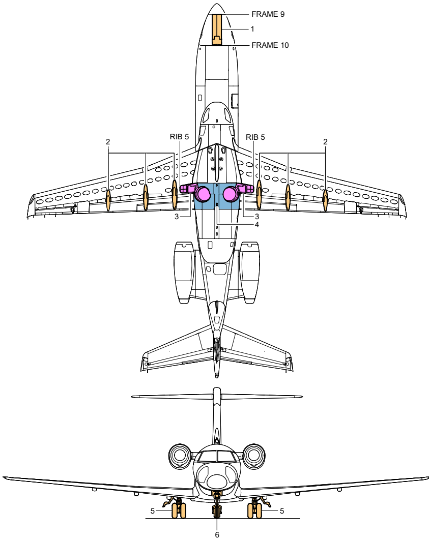
Figure 2-14-1: Unpaved runway conditions - Scheduled inspection zones
