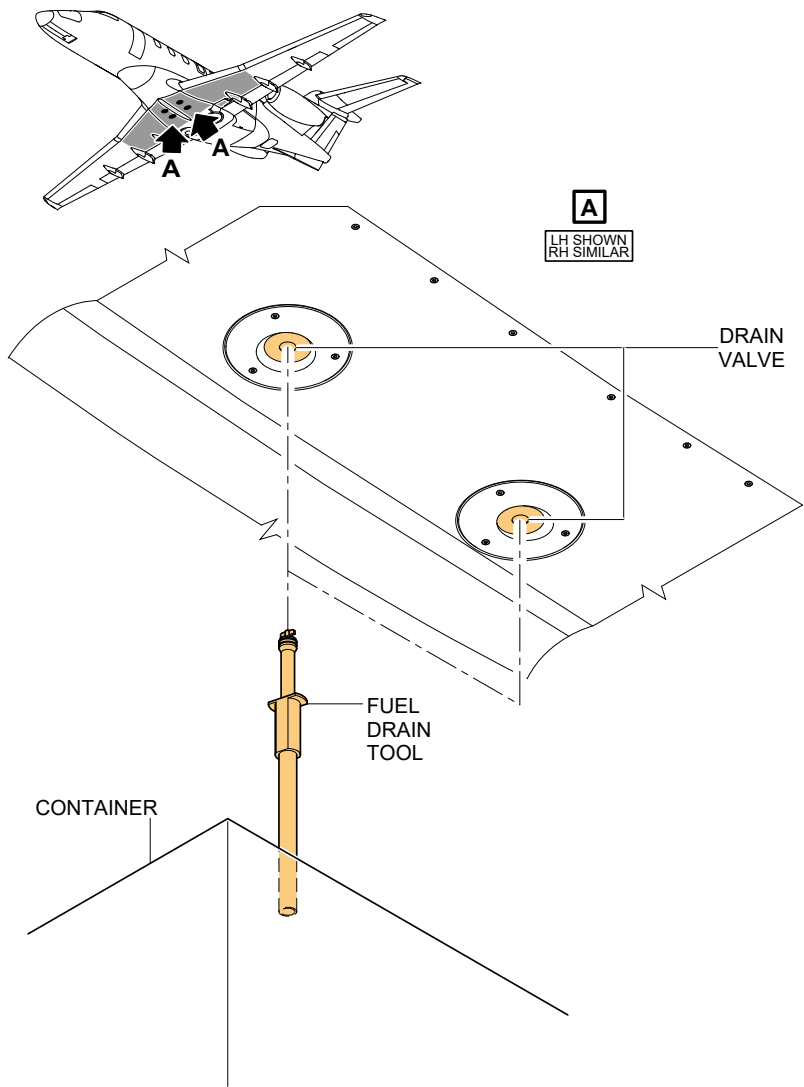
Figure 2-4-3: Fuel Drain Tool
