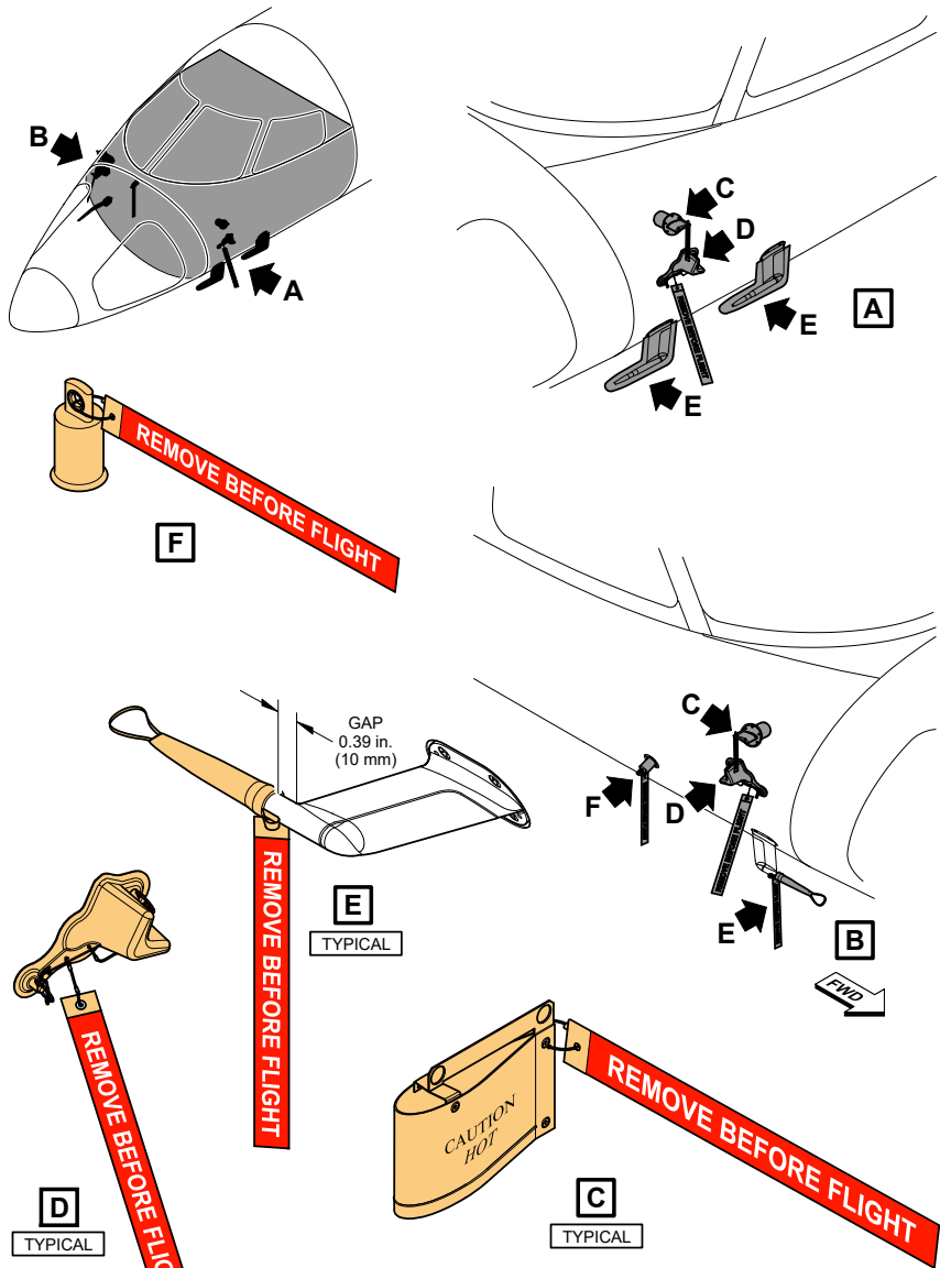
Figure 2-8-3: Parking - Air Data Probe Covers
