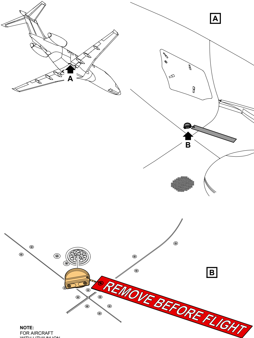
Figure 1-2-8: Parking - Lithium Ion Battery 2 - Vent cover
