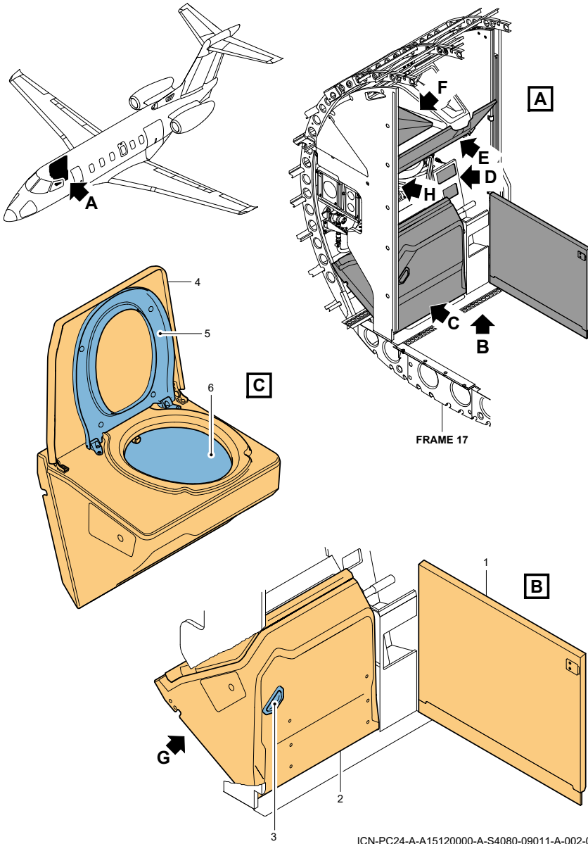
Figure 2-12-1: Water and waste system - Clean (Sheet 1 of 4)
