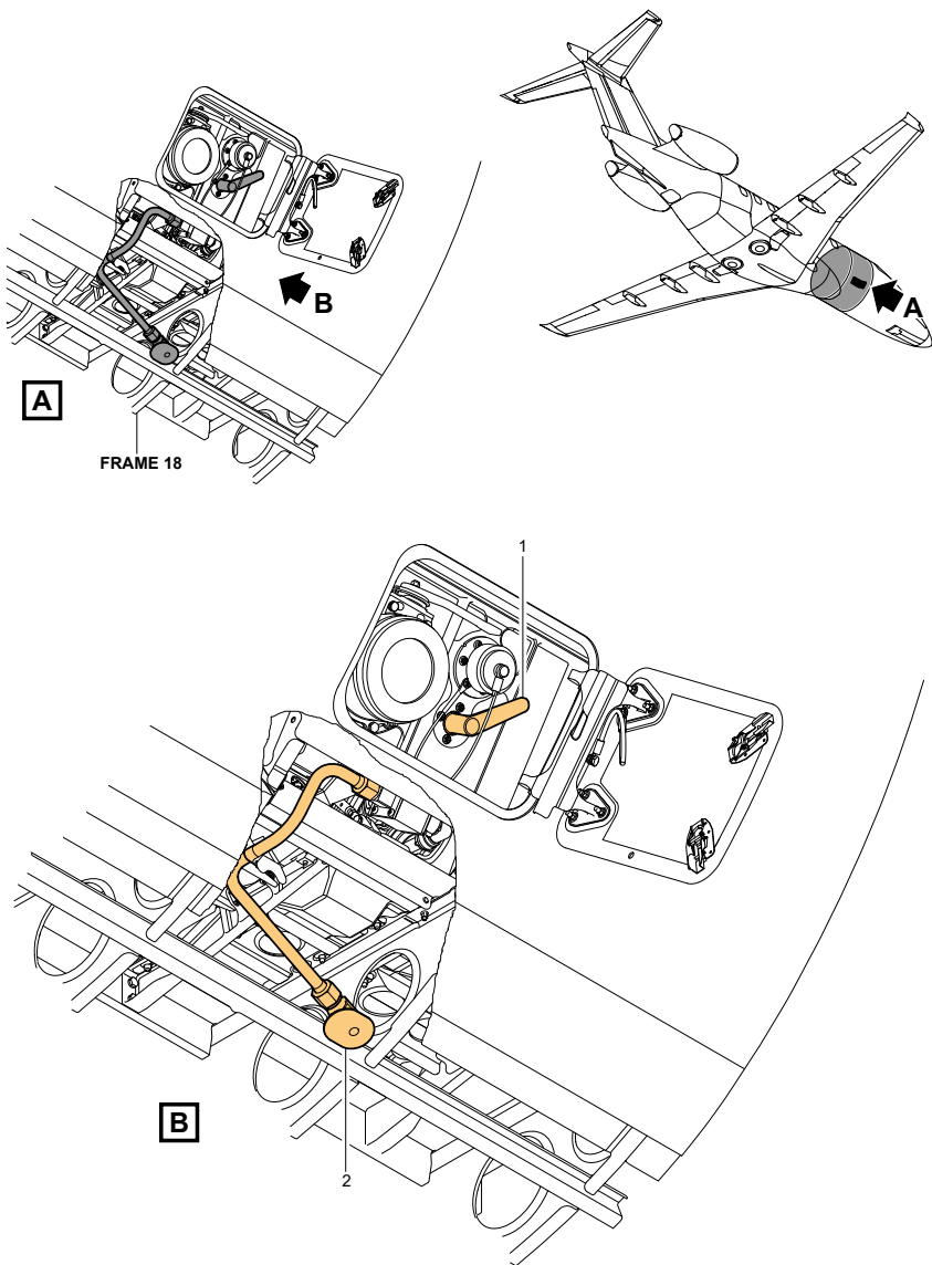
Figure 2-11-3: Water tank - Drain
