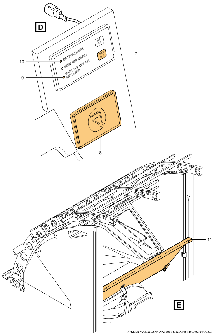
Figure 2-12-1: Water and waste system - Clean (Sheet 2 of 4)
