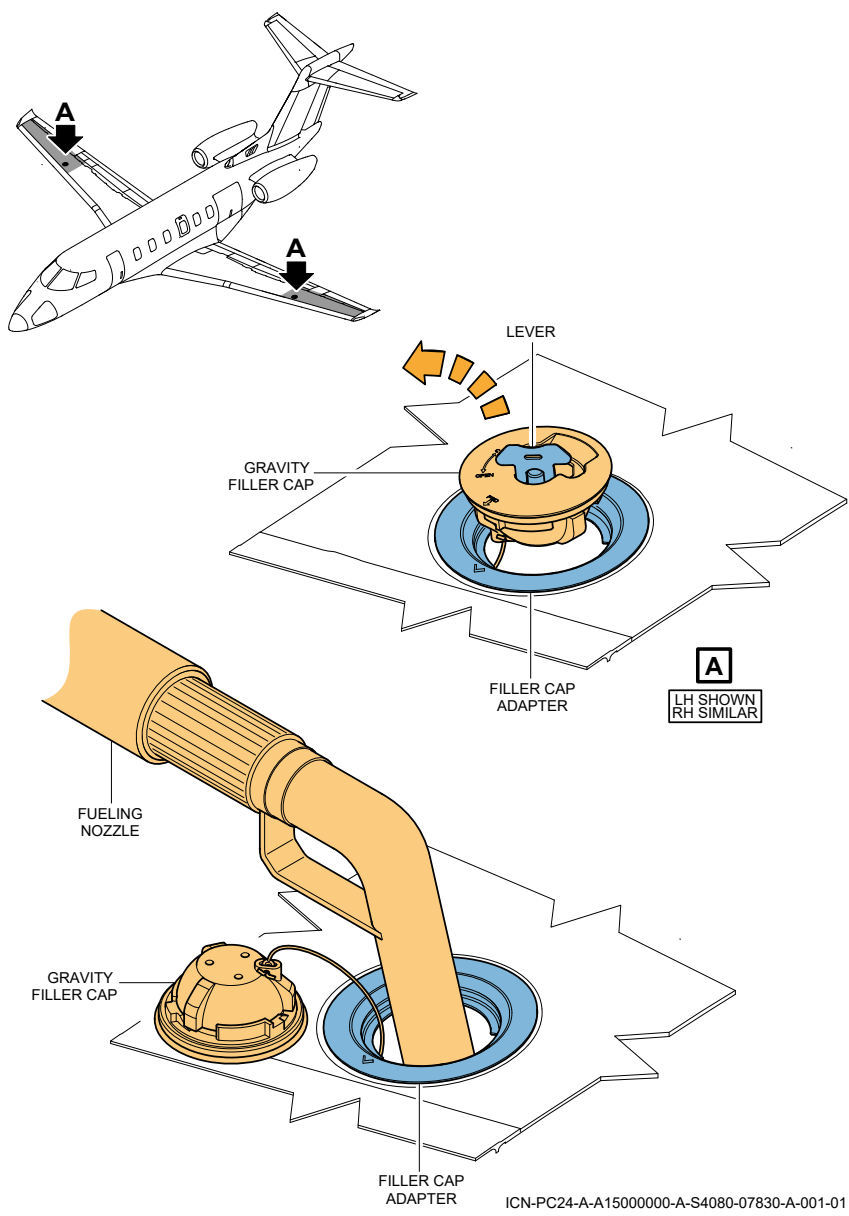
Figure 2-5-4: Fuel - Refuel by Gravity
