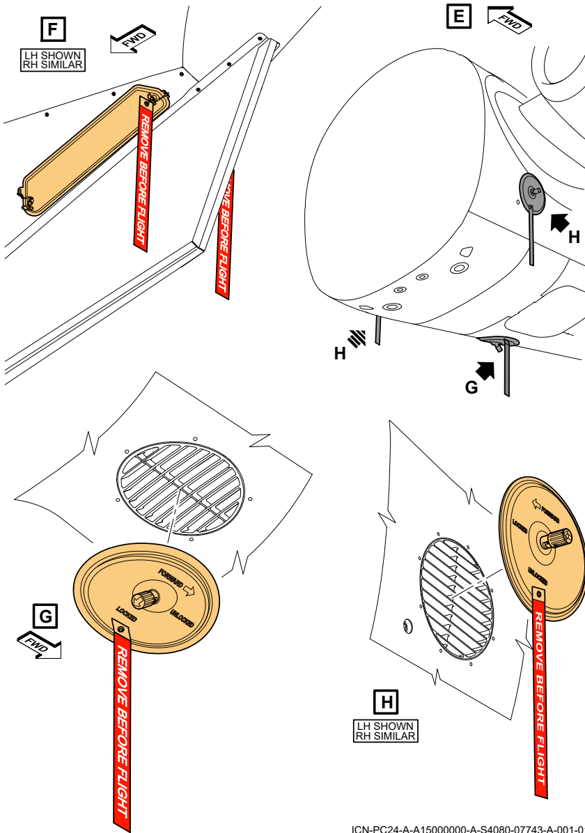
Figure 2-8-2: Parking - Lower Rear Fuselage Covers
