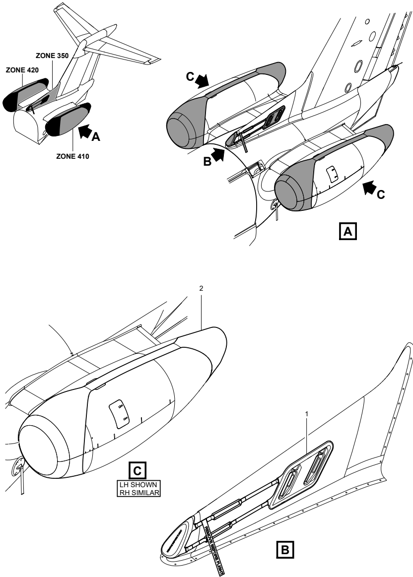
Figure 2-9-1: Water rinse - Exterior covers, aft
