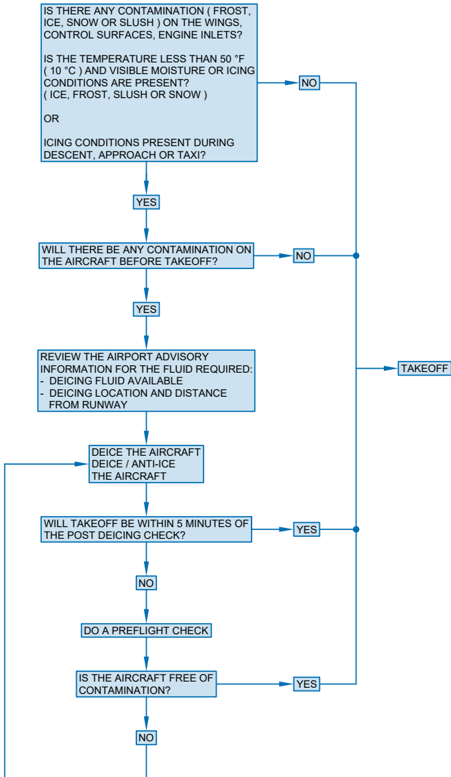
Figure 2-13-1: Deicing / Anti-icing Flowchart
